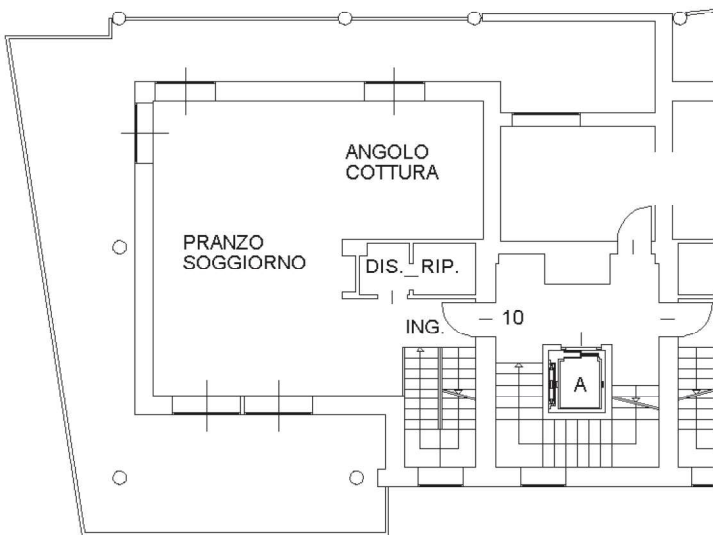
PIANO QUINTO h.2.70m
