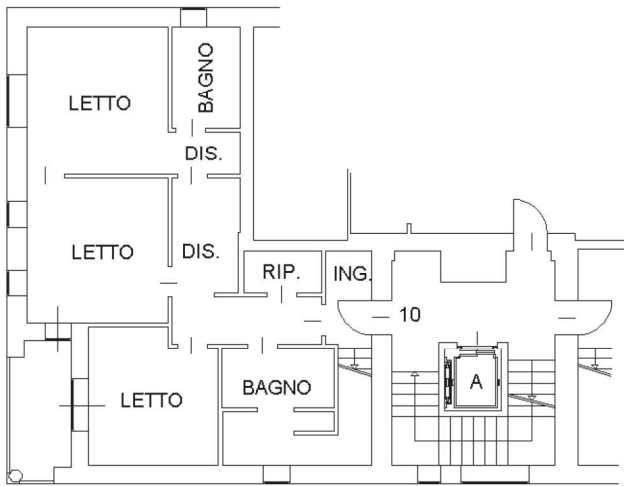
PIANO QUARTO h.2.70m
